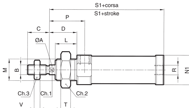
TIPO CT...1 (attacco post. radiale) CT...1 TYPE (radial rear mounting)
